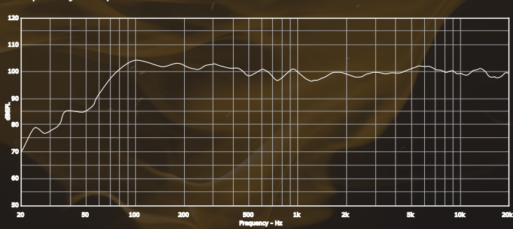
Frequency Response: QM4
